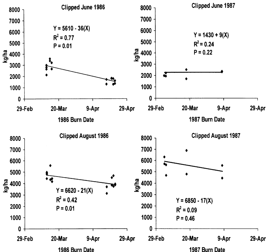
Fig. 1. Total herbage produced following dormant-season fires in moderately grazed tallgrass prairie in northcentral Oklahoma as measured on 2 dates in the first growing season. The independent variable is Julian date. Calendar dates are presented on the x-axes to aid interpretation. The slope coefficients of the equations for 1987 were not significant ( P > 0.05 ).
